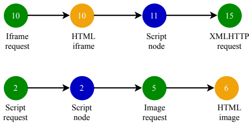
(a) Graph representation of Code 1 in ADGRAPH
