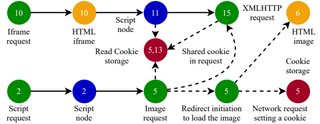
(b) Graph representation of Code 1 in WEBGRAPH
